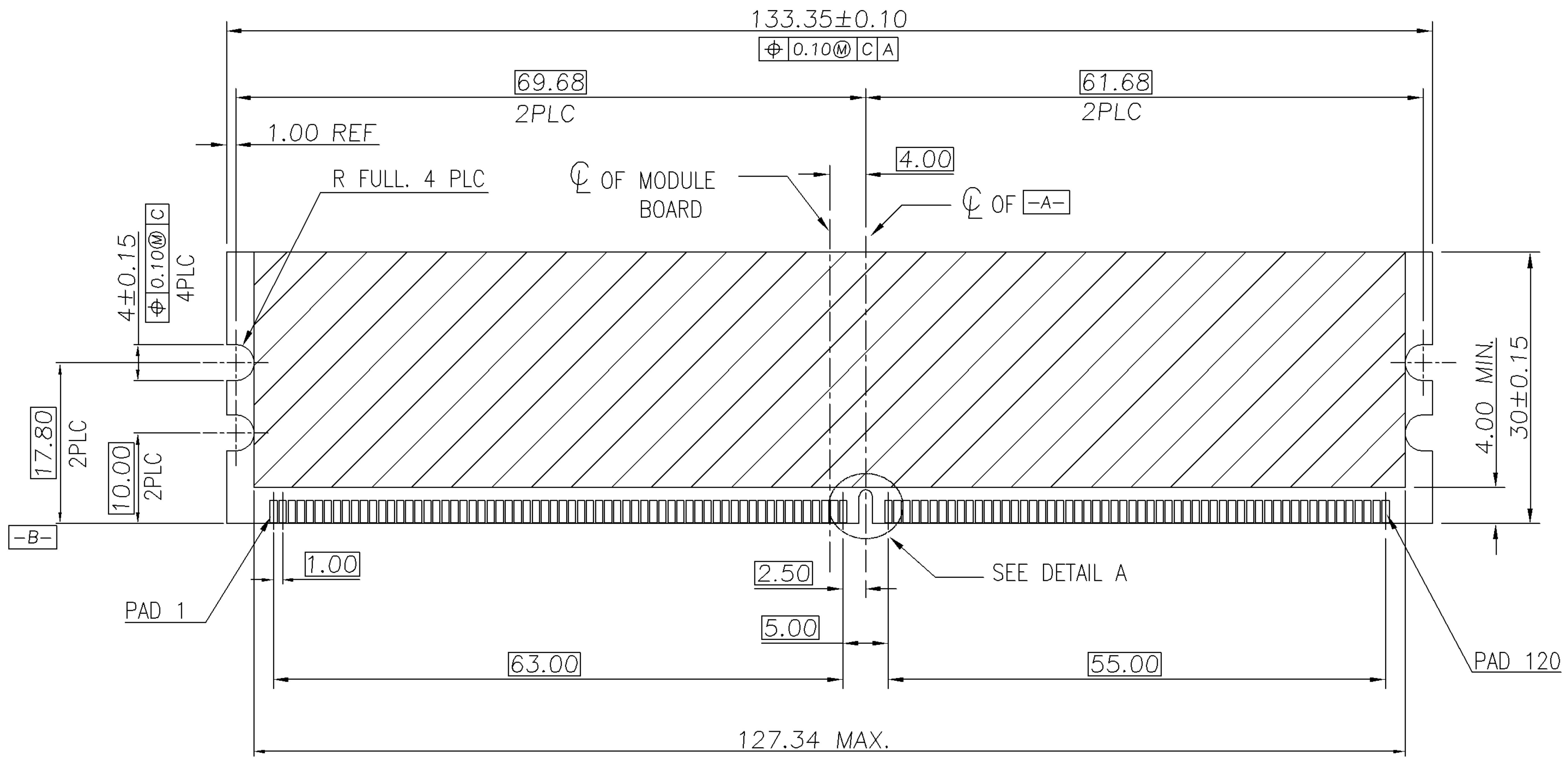
PLUG COMPONENT:DDR II 240P FUNCTION CARD
