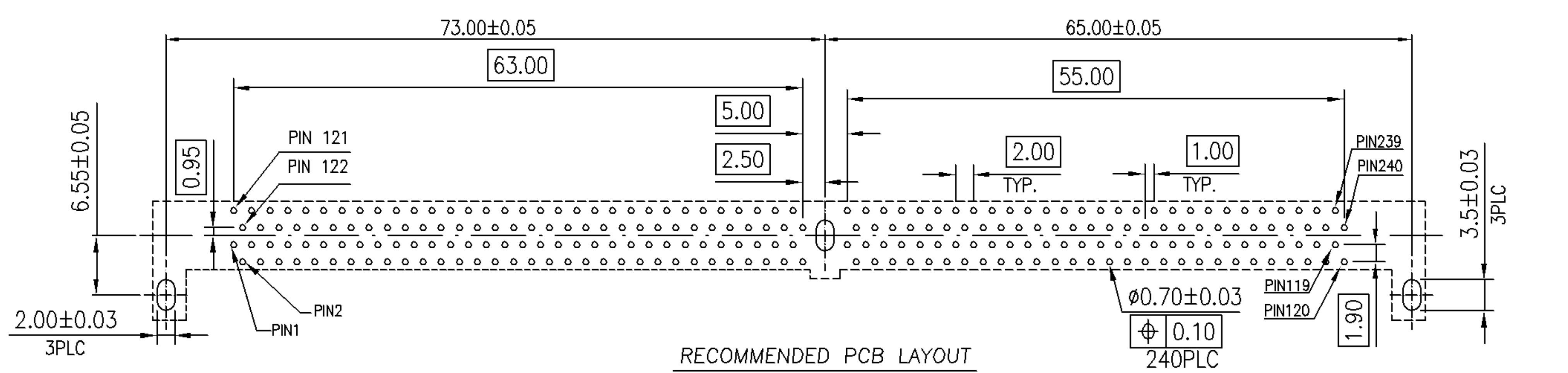
RECOMMENDED PCB LAYOUT
