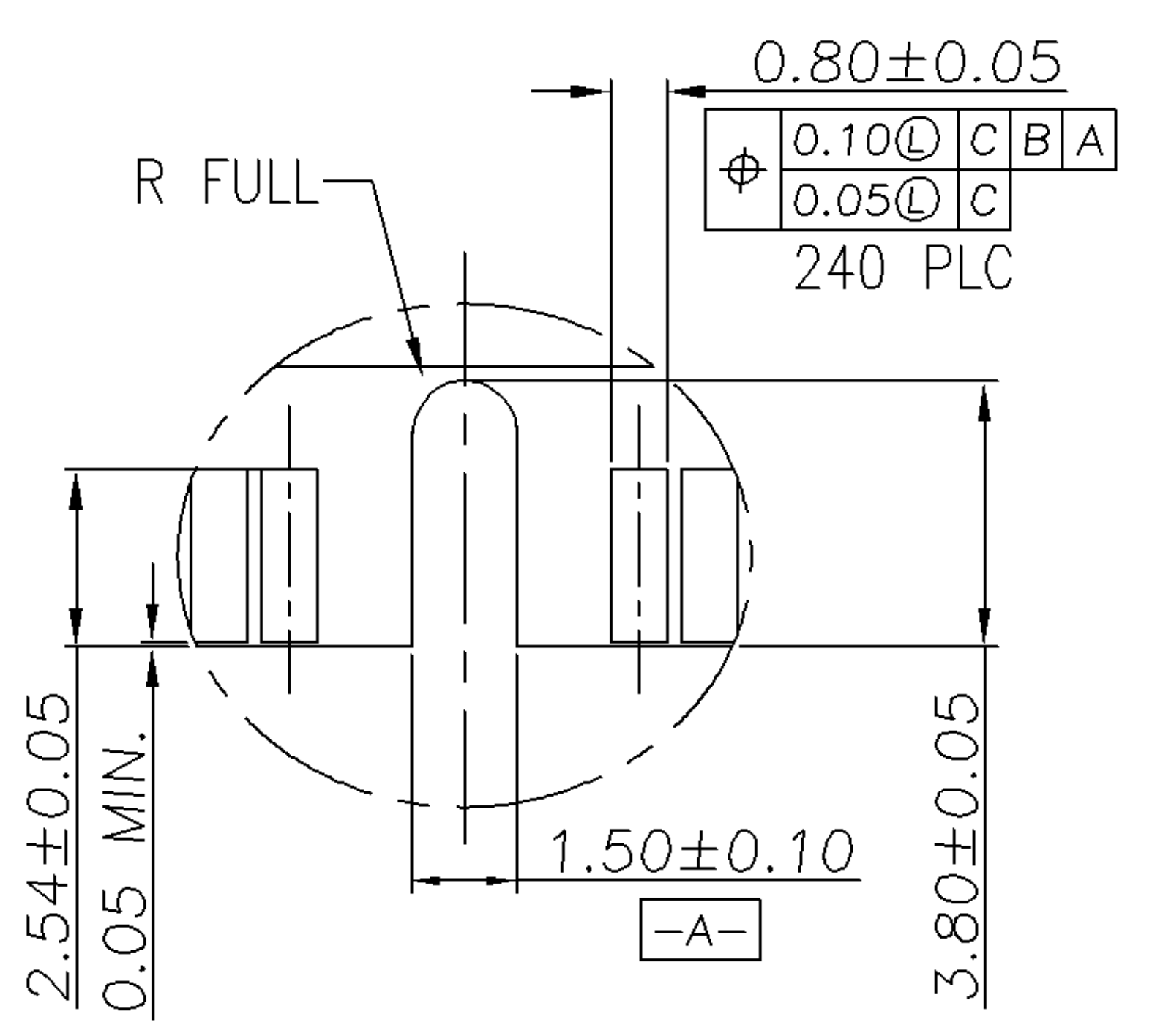
DETAIL A SCALE 3:1 (1.8V)
